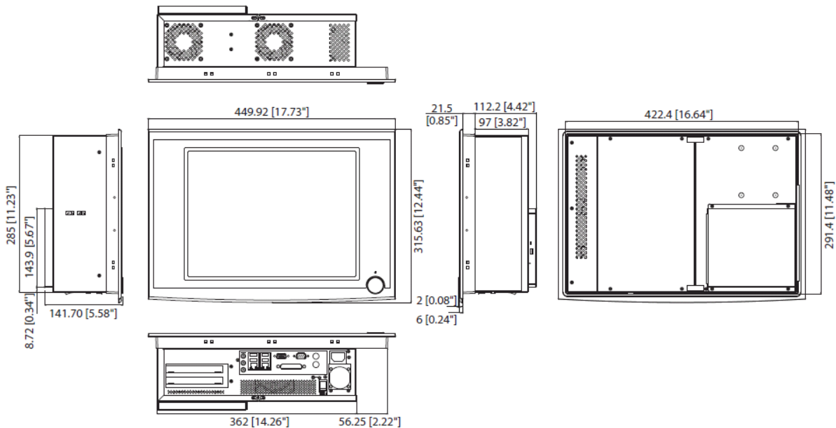
Panel Cut-out Dimensions: 428x297mm
